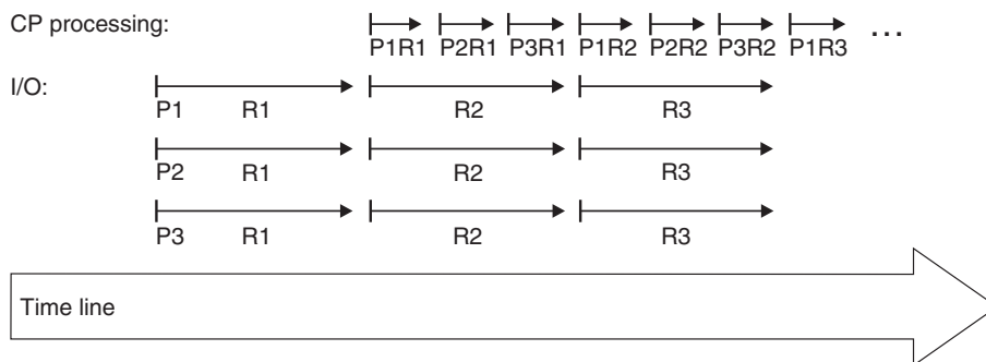
Figure 47. CP and I/O processing techniques. Parallel I/O processing.
