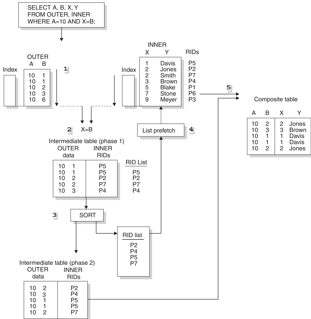
Figure 86. Hybrid join (SORTN_JOIN='Y')
