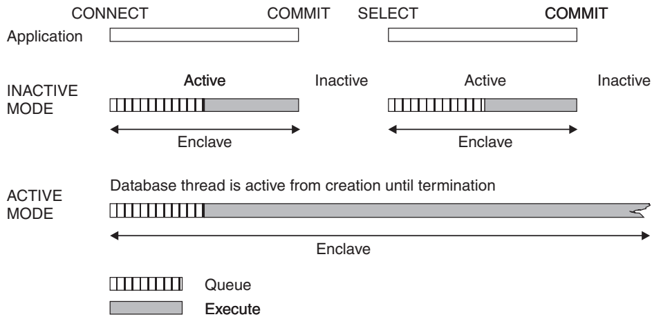
Figure 69. Contrasting ACTIVE MODE threads and POOLED MODE threads
